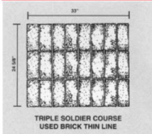
SOLDIER COURSE USED BRICK THIN LINE
